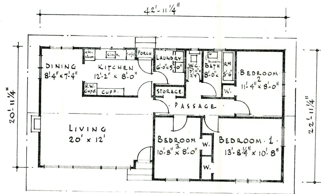
FLOOR PLAN
